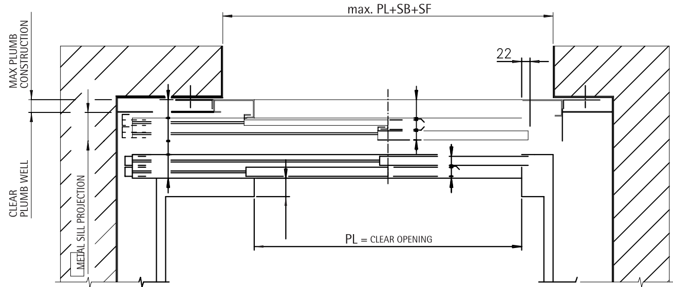
NICHE INSTALLATION
